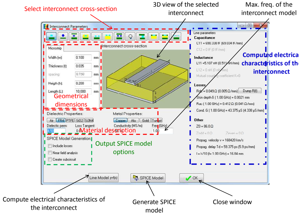
Figure 4- 39: Interconnect R,L,C model based on physical dimensions
