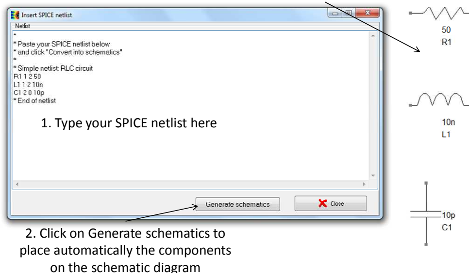
Figure 4- 14: Type a SPICE netlist and insert the components on the schematic diagram ("Insert > Insert Netlist")
