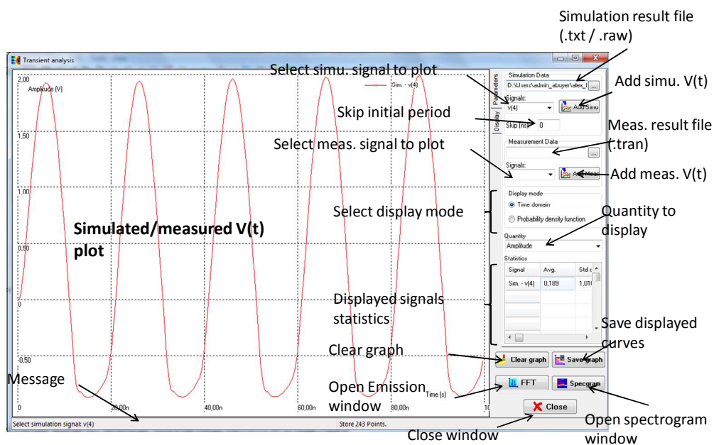
Figure 4- 24: Time-domain profile of the signal under investigation (case_study\s12x\s12x_RFI_pt3_iosupply_tran.sch)
