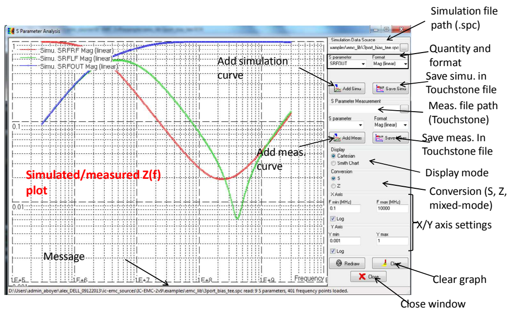
Figure 3- 22: S parameter simulation of a three port bias tee (examples\EMC_lib\3_port_bias_tee.sch)
