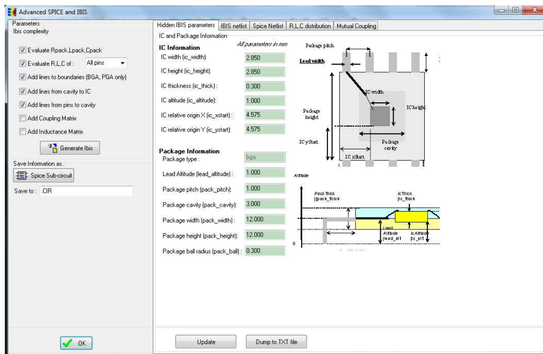
Figure 4- 34: the user's interface for the Advanced Spice and Ibis Information
