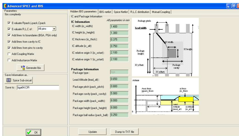
Figure 3- 76: Module “Advanced SPICE and IBIS” on a BGA (examples\ibis\BGA64.ibs)
