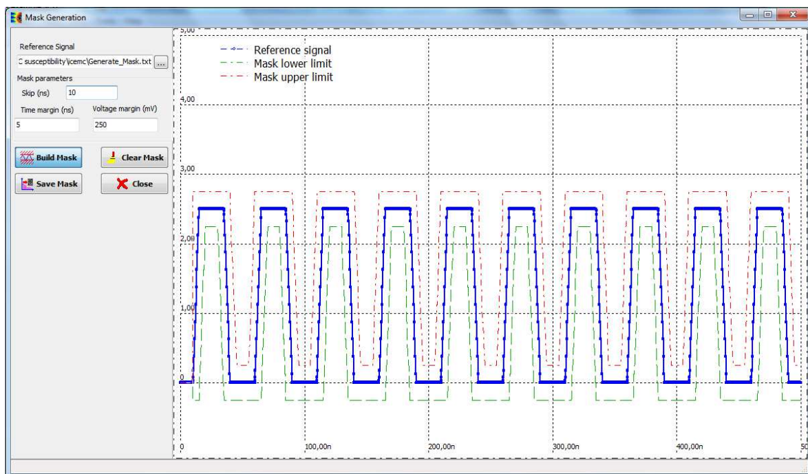
Figure 4- 33: Generation of a mask for failure detection during susceptibility simulation
