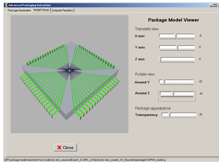
Figure 4- 37: 3D view of the advanced package (examples\package\TQFP64.geo)
