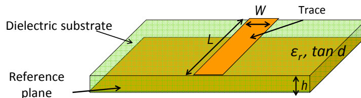
Figure 3- 64: Geometry of the modeled microstrip line
