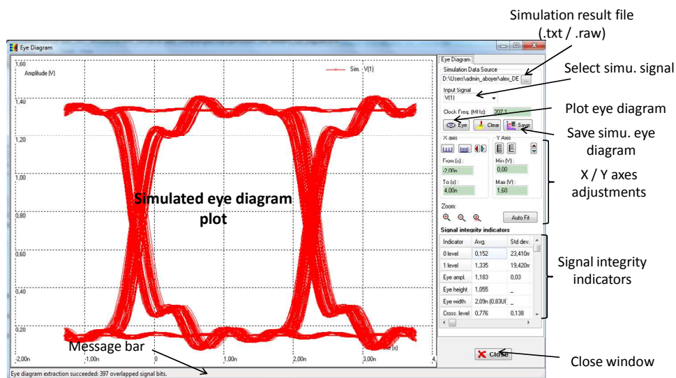
Figure 4- 47: Eye diagram plot (basic\signal_integrity\ Eye_digital_IO_switching.sch)
