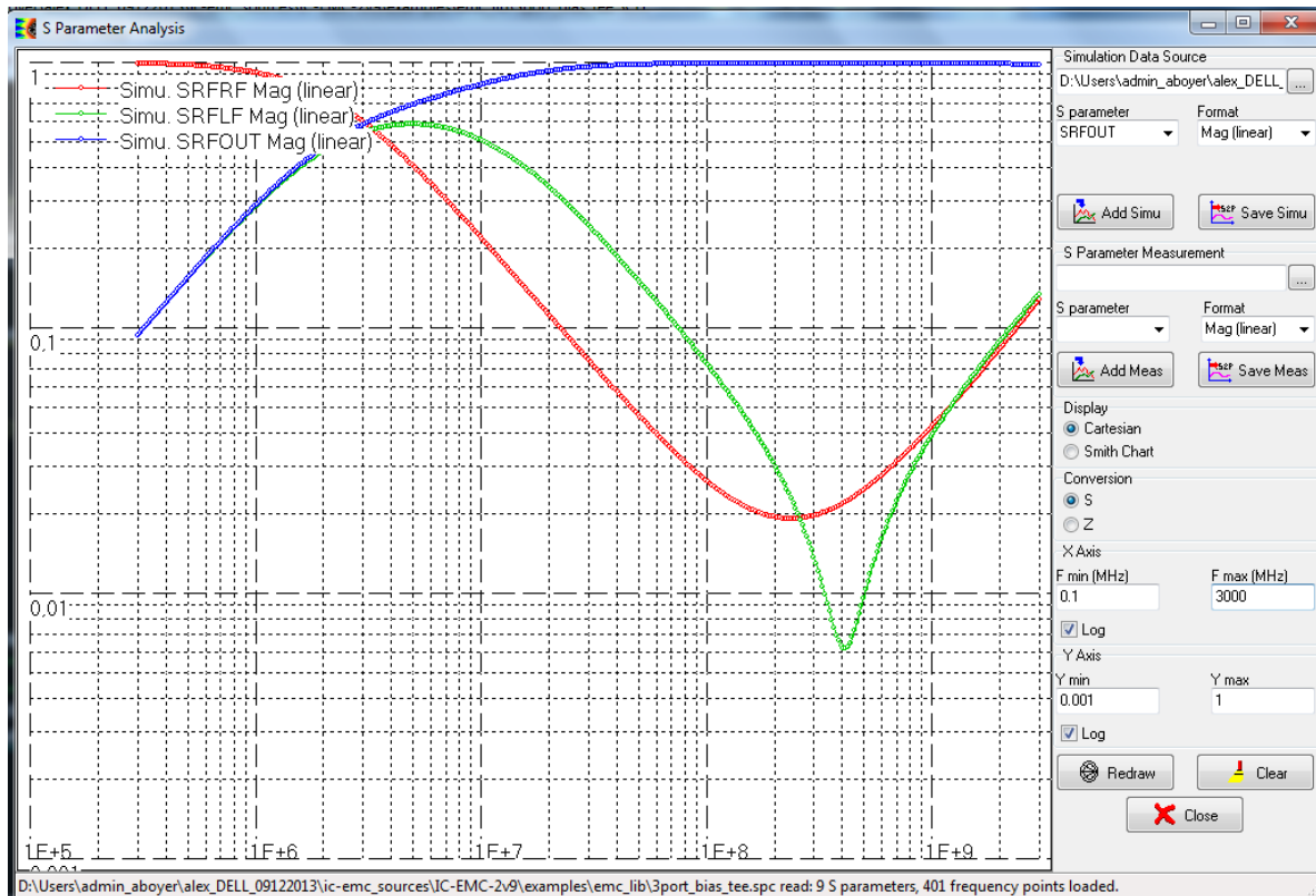
Figure 4- 28: S parameter analysis user's interface (examples\EMC_lib\3port_bias_tee.sch)
