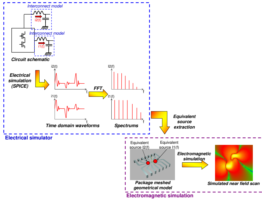
Figure 3- 53: General simulation flow for IC radiated emission prediction
