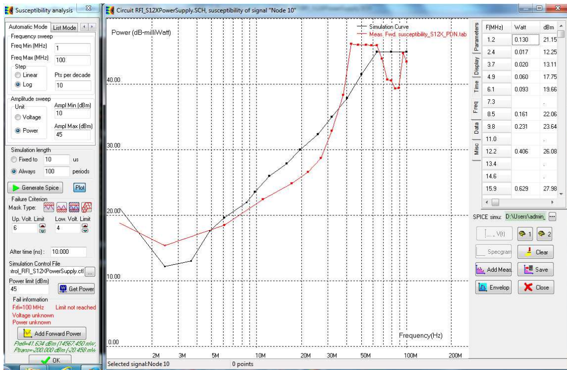
Figure 3- 29: Comparison between measurement and simulation of the susceptibility threshold of the S12X microcontroller (examples\immunity\S12X_RFI\RFI_S12XPowerSupply.sch)
