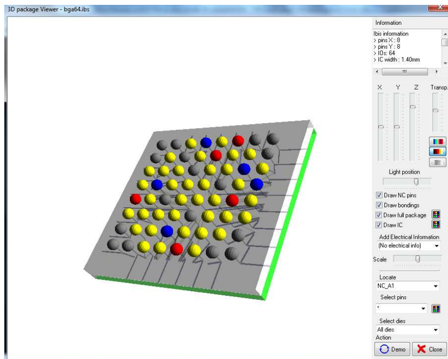
Figure 4- 35: the 3D-package viewer (examples\ibis\bga64.ibs)
