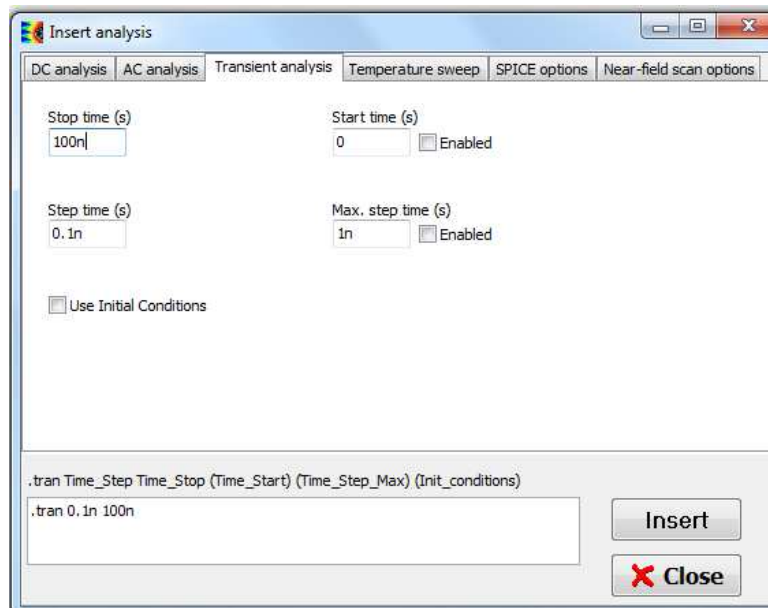
Figure 2- 16: Define the SPICE analysis
