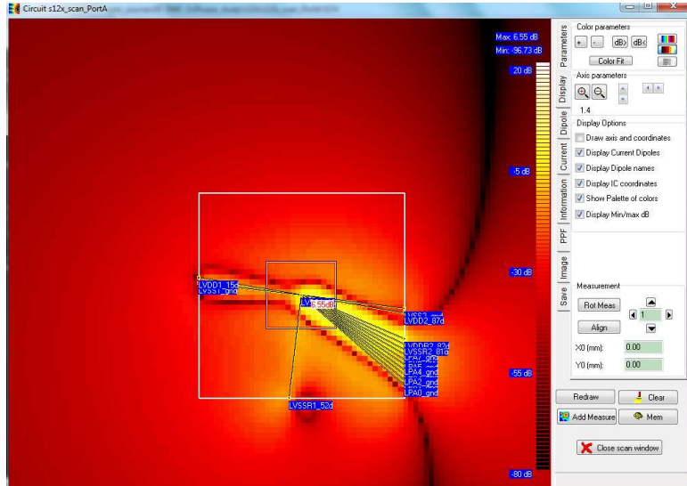
Figure 4- 21: The near-field scan user's interface (case_study\s12x\s12x_scan_portA.sch)
