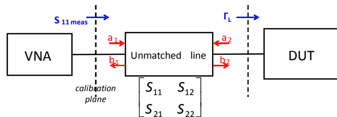
Figure 4- 43: The DUT input is connected to the VNA by a unmatched line fully characterized
