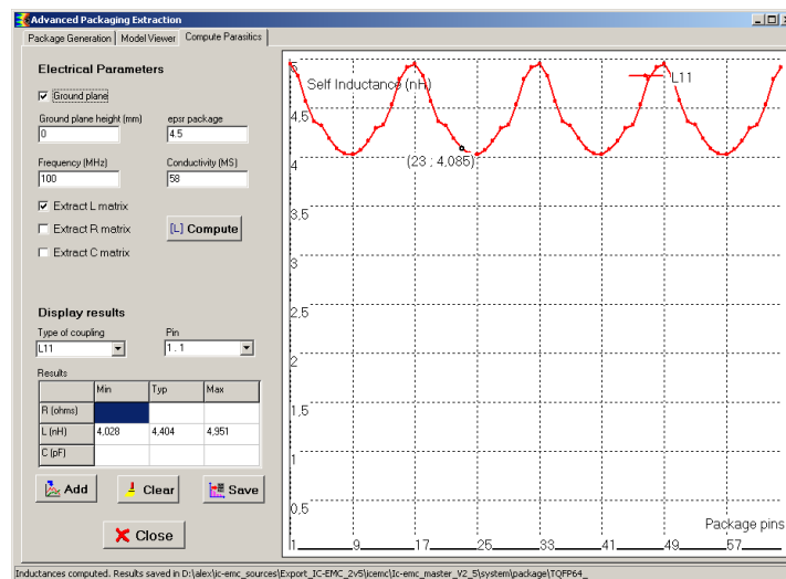
Figure 4- 38: Interface for computation and display of package electrical parasitics (examples\package\TQFP64.geo)
