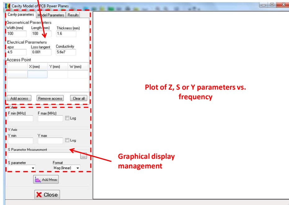
Figure 4- 41: Configuration of cavity dimensions and port placement
