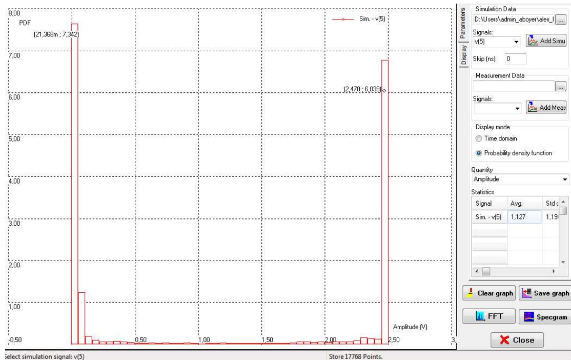
Figure 4- 26: Statistical distribution of the amplitude of the output voltage of a noisy inverter ( examples\transient\noisy_inverter.sch )
