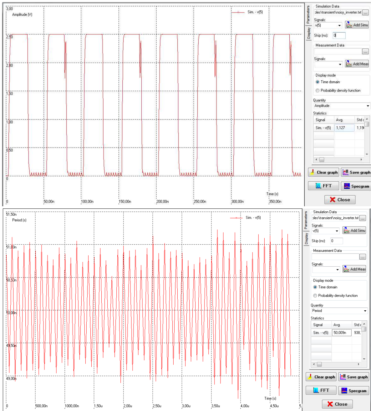
Figure 4- 25: Output voltage of a noisy inverter (top), and tracking of the period of its output signal (bottom) (examples\transient\noisy_inverter.sch)
