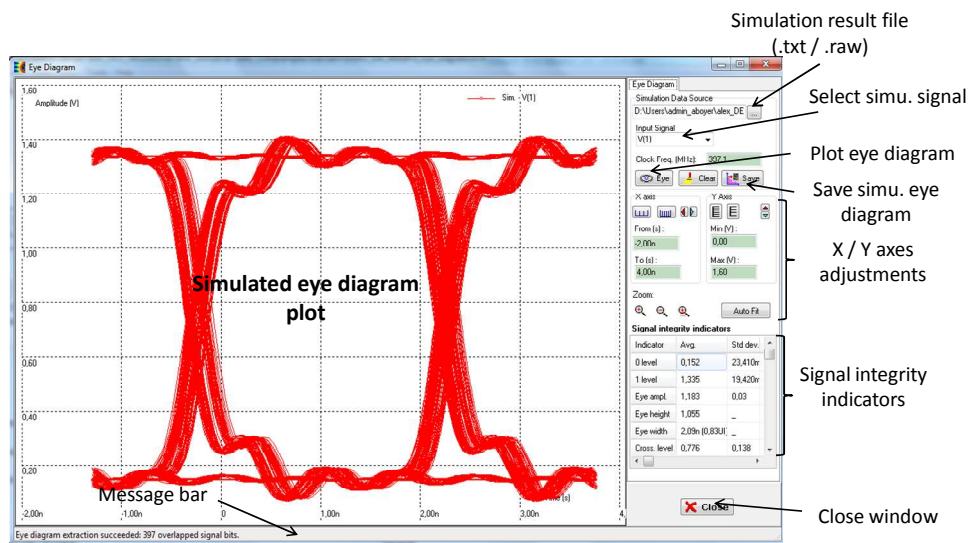
Figure 3- 50: Eye diagram of the DDR3 memory link (\\examples\\transient\\DDR3_link_400MHz_eye_diagram.sch)
