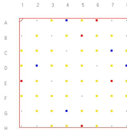
Figure 3- 77: 2D floorplan of a BGA 64 package (examples\ibis\BGA64.ibs)
