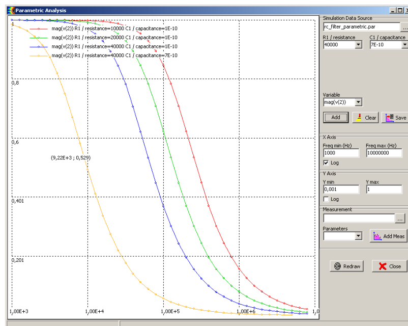
Figure 4- 30: Plot of the results of Parametric analysis (examples\misc\rc_filter_parametric.par)
