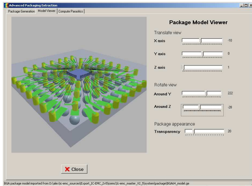
Figure 3- 98 : Constructed model of a BGA 64 (examples\package\ BGA_model.geo)
