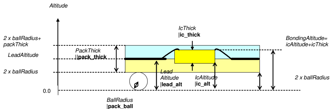
Figure 4- 19: Cross-section and main physical parameters describing a package
