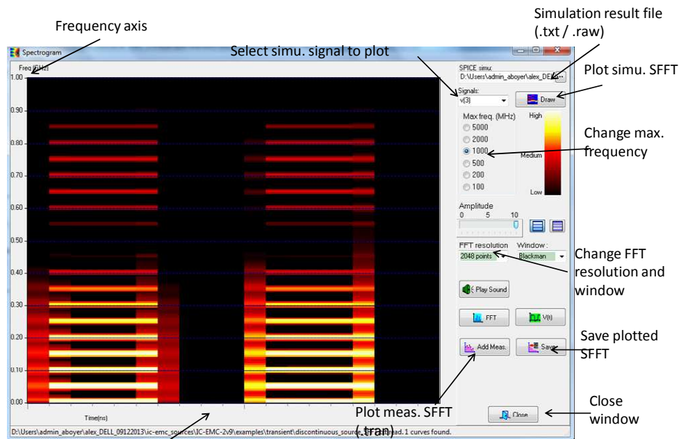
Figure 4- 46: Spectrogram user's interface (examples\transient\ discontinuous_source_SFFT.sch)
