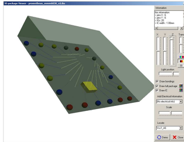
Figure 3- 59: 3D view of the PA package (\case_study\pa_3G\ prometheus_mmm6030_v2.ibs)
