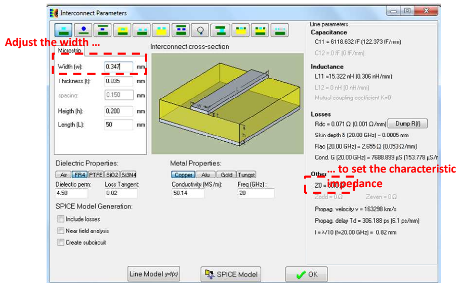
Figure 3- 66: Adjustment of the trace's width to set the characteristic impedance of the microstrip line
