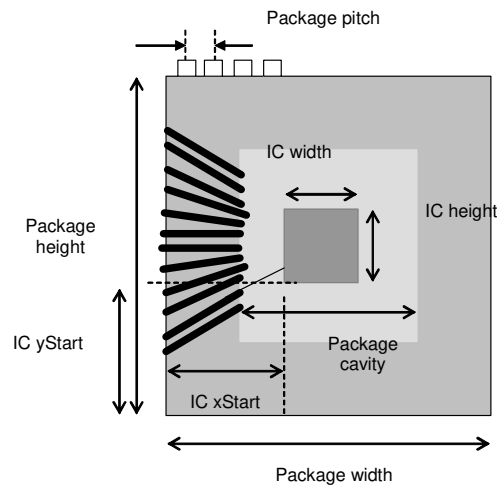
Figure 4- 18: Top view of the package
