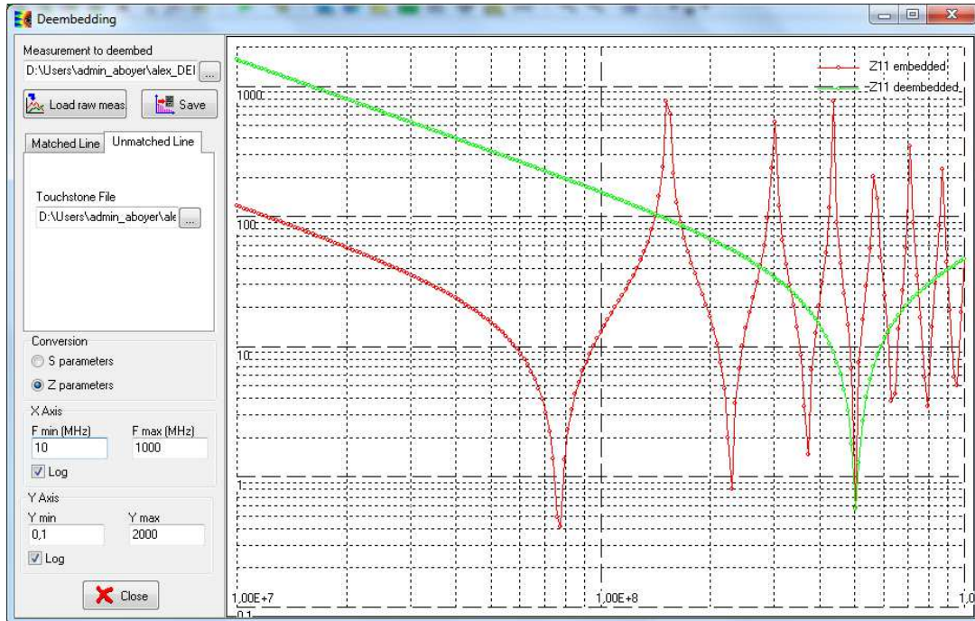
Figure 4- 44: S parameter deembedding user's interface (examples\basic\deembed\S11_rawDeembed.s1p)
