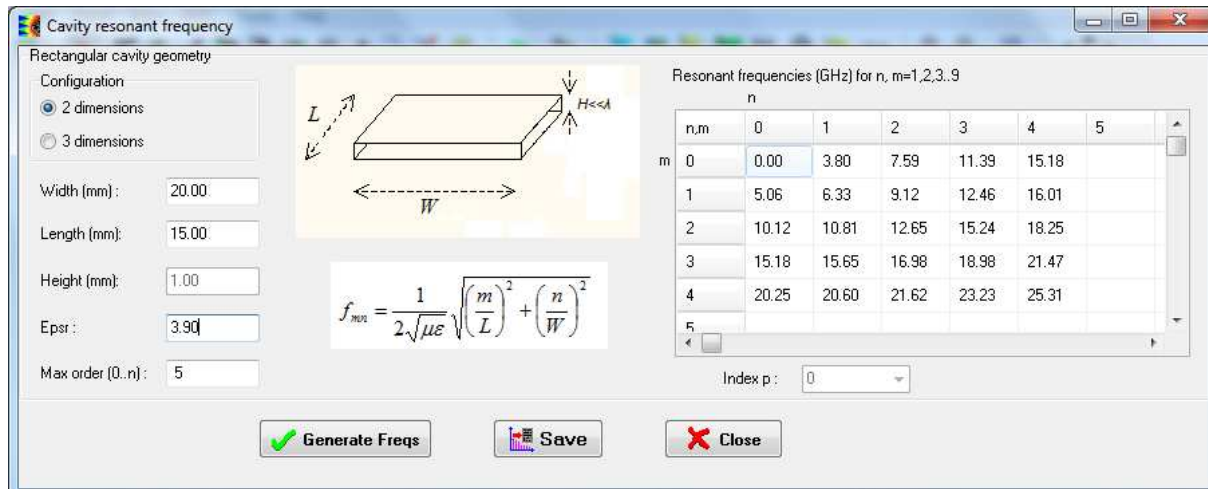
Figure 4- 51: Computation of the resonant frequencies of a rectangular 2D/3D cavity
