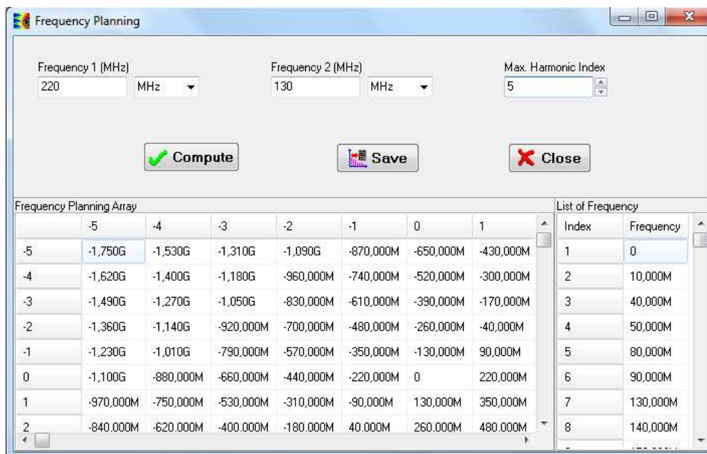
Figure 4- 52: Calculation of the frequencies of intermodulation products between 2 harmonic signals
