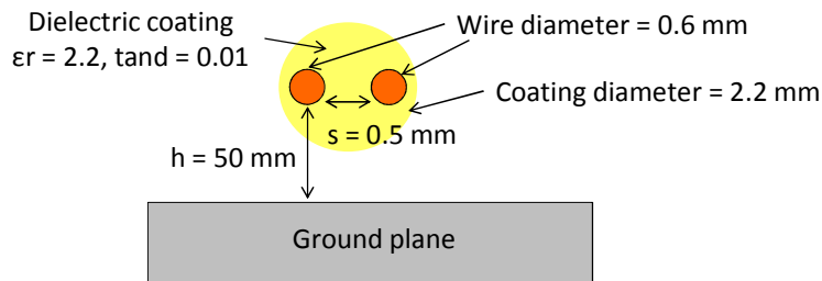
Figure 3- 72: Geometry of the modeled cable
