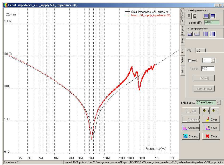
Figure 4- 27: The Z(f) screen with frequency-domain simulations (examples\impedance\Impedance_c51_supply.sch) compared to measurements (examples\impedance\c51_supply_impedance.s50)
