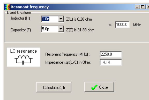
Figure 4- 48: Resonant frequency of given L and C, with associated impedance
