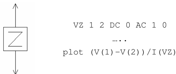
Figure 3- 12: Impedance probe and associated SPICE description
