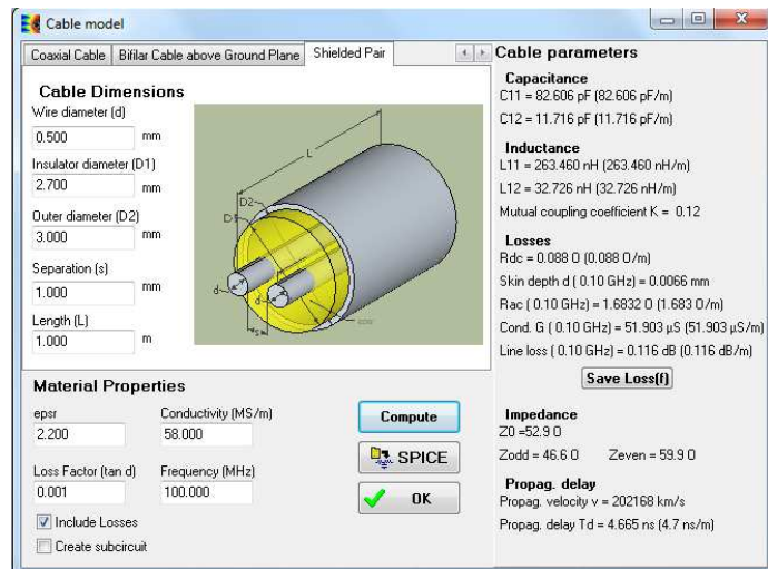
Figure 4- 40: The attenuation in cable evaluation interface
