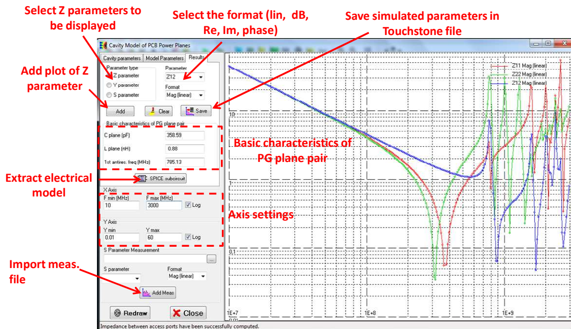
Figure 4- 42: Cavity resonator model: A result plot
