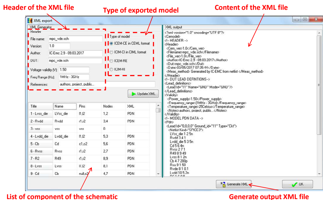
Figure 4- 7: Export of a schematic diagram in a XML file (examples\emission\mpc\mpc_vde.sch)
