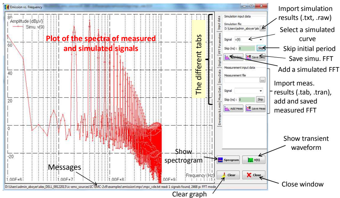
Figure 4- 20: the window "Emission vs. Frequency"
