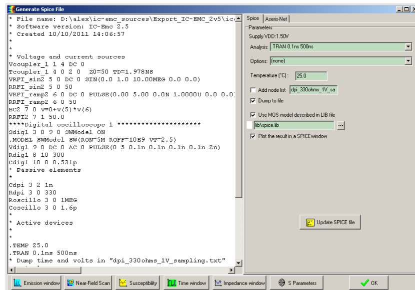
Figure 4- 16: Converting a schematic diagram into a SPICE-compatible text file
