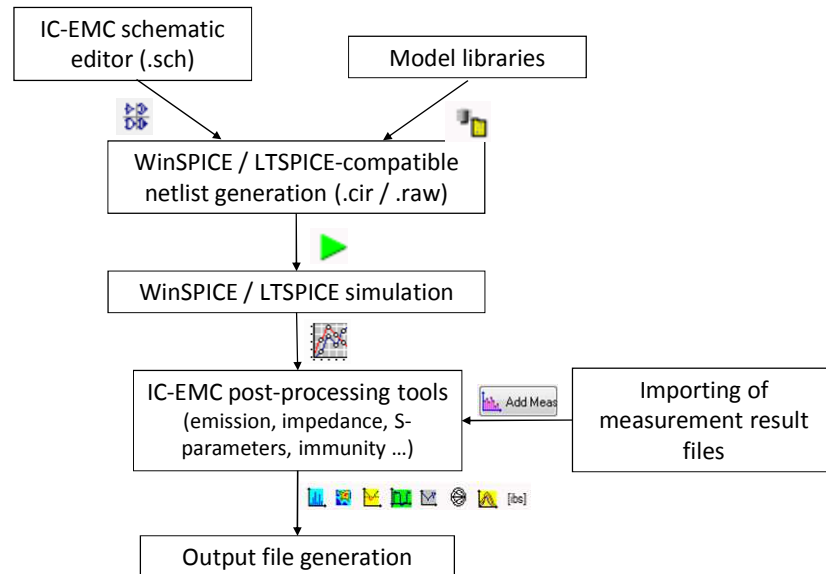
Figure 2- 3: General simulation flow with IC-EMC
