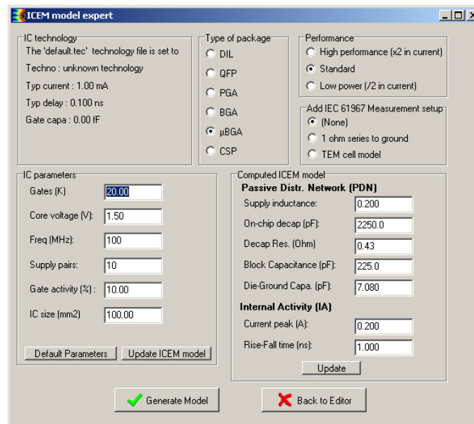
Figure 4- 31: The ICEM model generator and its user's interface
