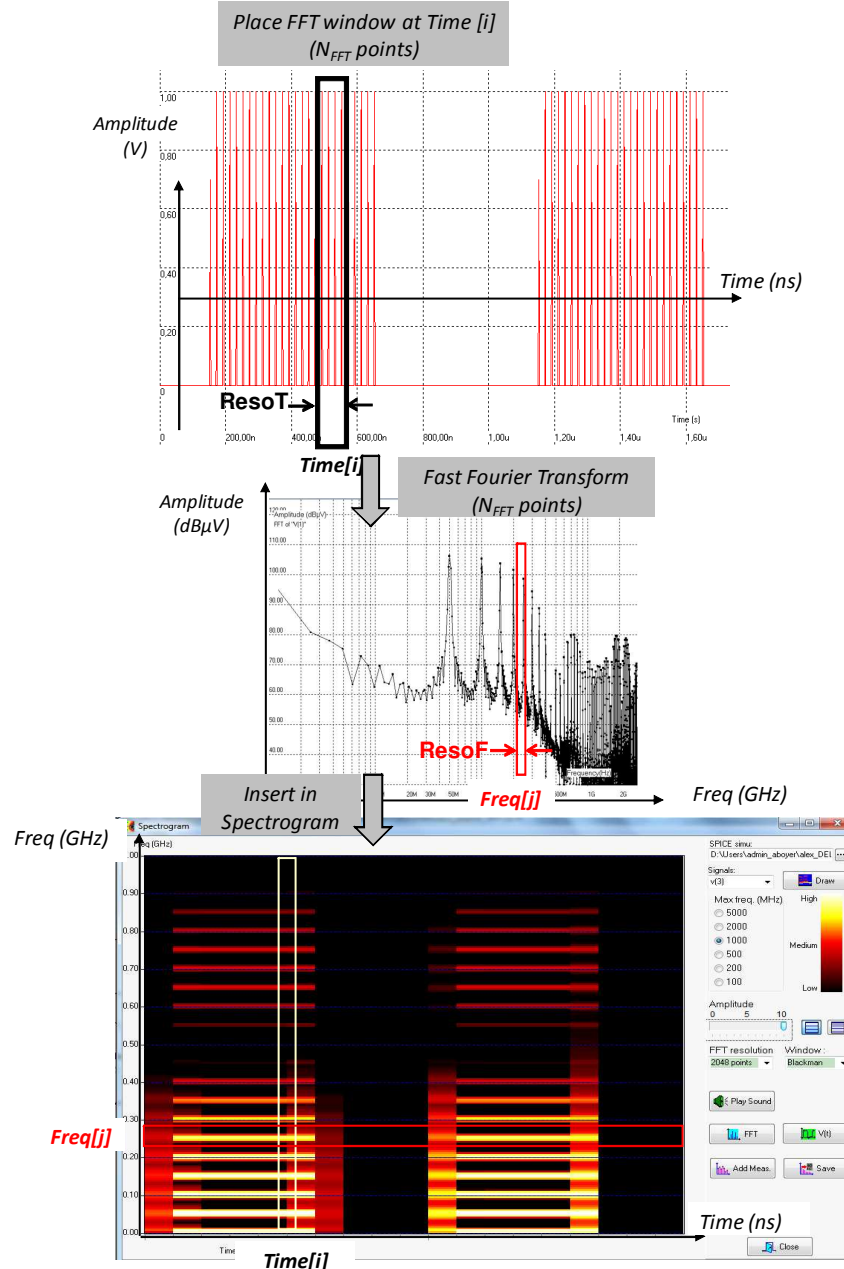
Figure 4- 45: Spectrogram principles (examples\transient\ discontinuous_source_SFFT.sch)
